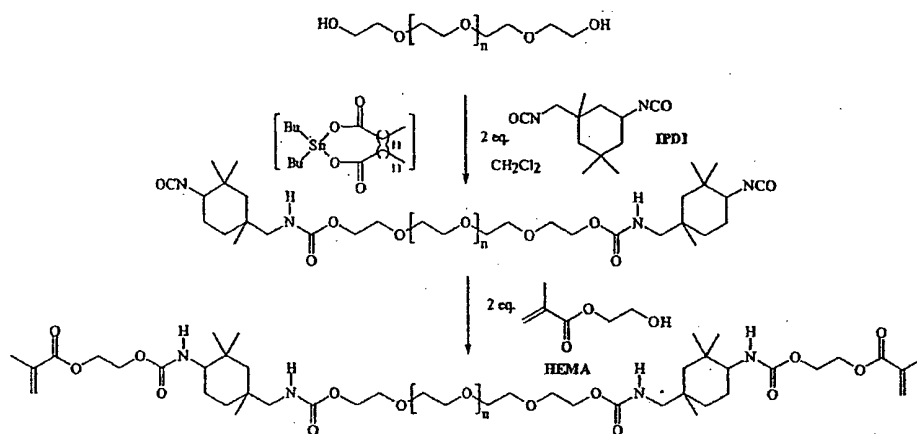
Fig. 1: Two-step-one-pot synthesis of vinyl-terminated polyethyleneoxides
